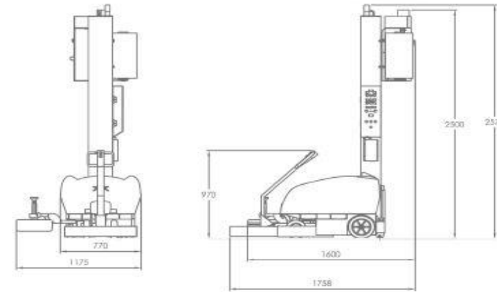
Machine Dimensions
